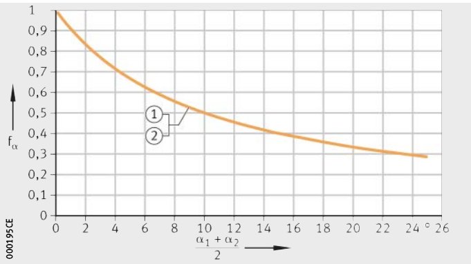
Figure 25 Correction factor for tilt angle
