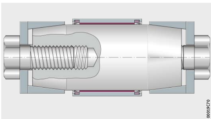
Figure 3 Ready-to-fit system with ELGOGLIDE® plain bushes
