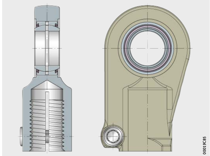
Figure 15 Special rod end for fork lift trucks
