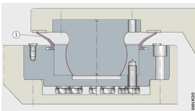
Figure 14 Central joint bearing
