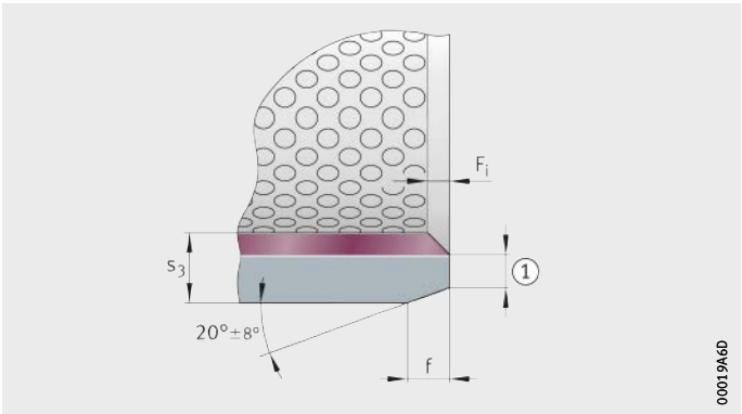
Figure 3 Outer chamfer and inner edge break
