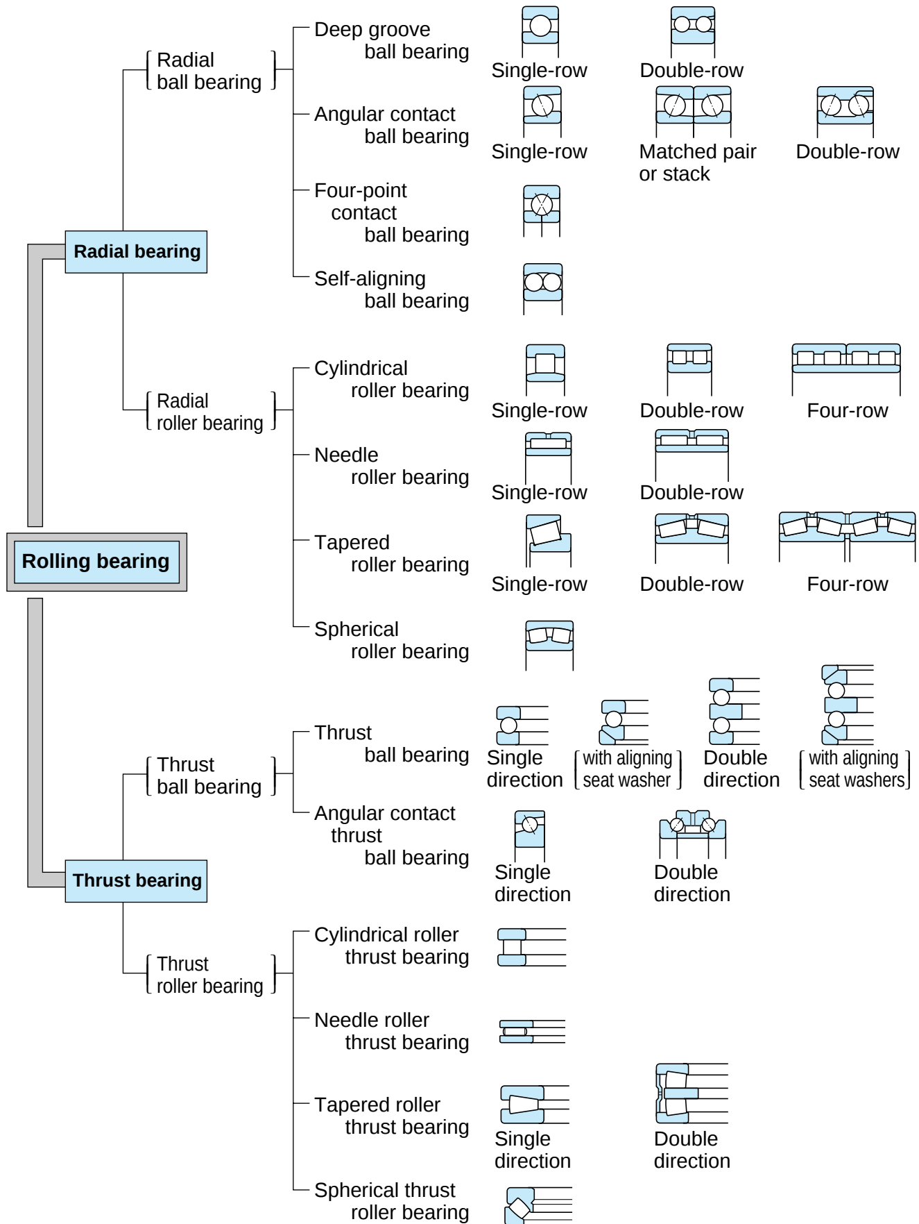
Fig. 1-2 Rolling bearings
