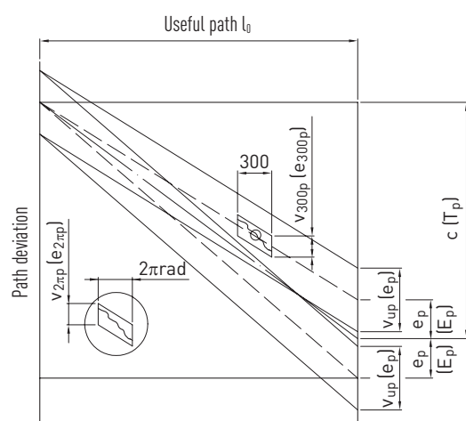
Fig. 3.12 HIWIN measurement curve of lead of precision ballscrews
