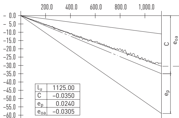
Fig. 3.15 Average path deviation over useful path l_u
