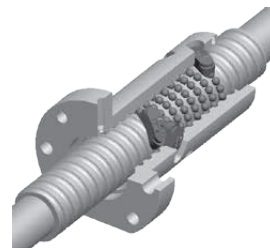
Fig. 3.10 Internal single recirculation type nut
