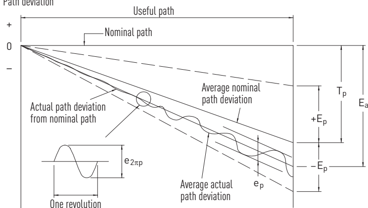
Fig. 3.12 HIWIN measurement curve of lead of precision ballscrews
