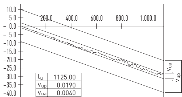
Fig. 3.16 Travel fluctuation over useful path l_u
