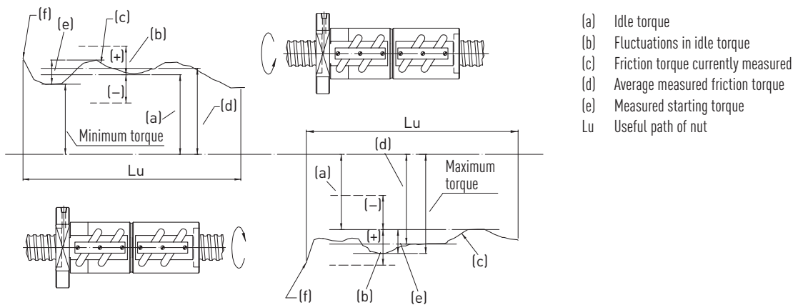
Fig. 3.21 Nomenclature for measuring idle torques
