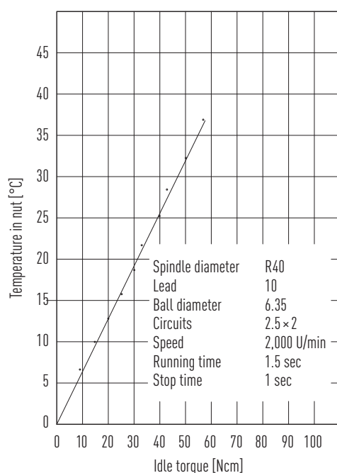
Fig. 3.29 Relationship between temperature increase in the ballscrew and idle torque
