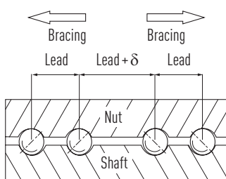
Fig. 3.19 Preload from lead offset
