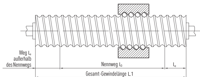
Fig. 3.13 DIN ISO measurement curve of lead of ballscrews
