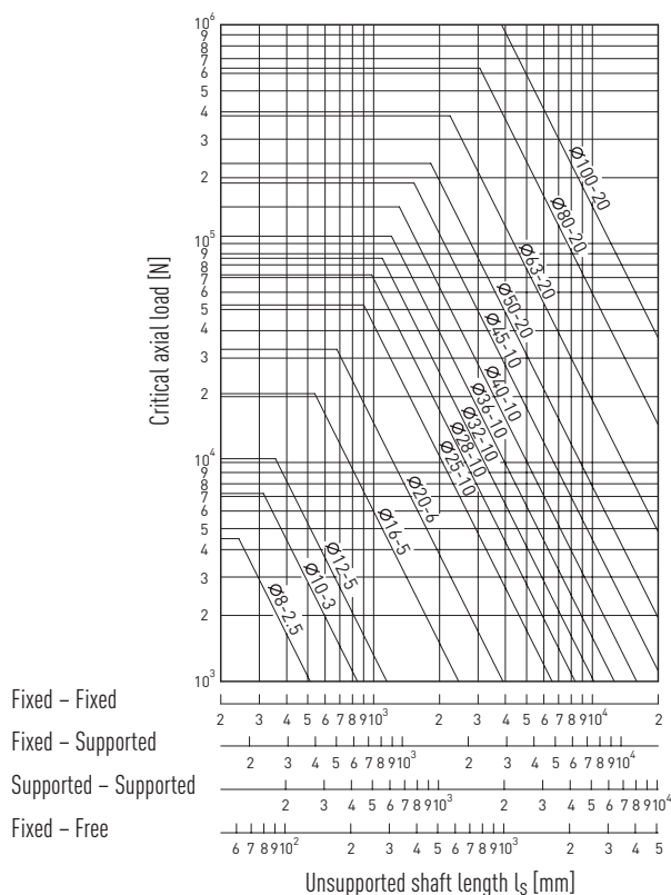
Fig. 3.24 Buckling load for different diameters and lengths of threaded shafts
