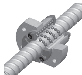
Fig. 3.11 Endcap recirculation type nut
