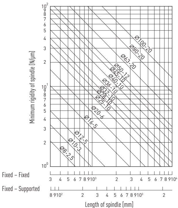
Fig. 3.26 Rigidity diagram for ballscrews
