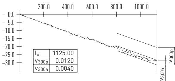
Fig. 3.14 Travel fluctuation over 300 mm useful path
