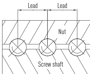
Fig. 3.18 Preload from ball size
