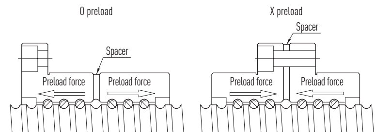
Fig. 3.20 Preload from spacer
