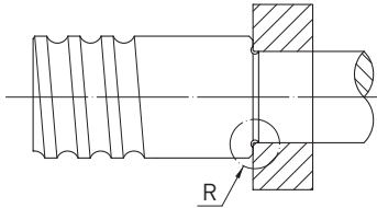
Fig. 3.7 Recess for positioning end bearings
