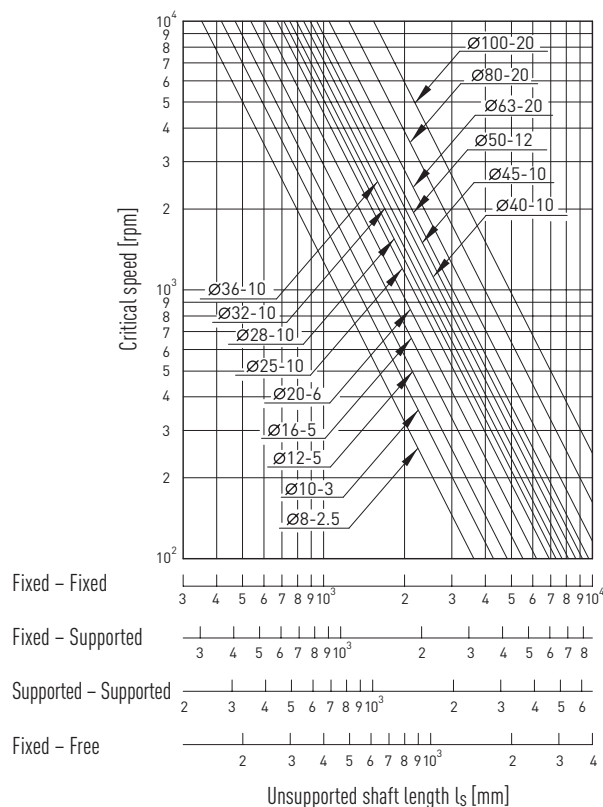
Fig. 3.25 Critical speed for different diameters and lengths of threaded shafts
