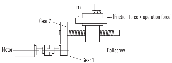
Fig. 3.22 Load trend of a system with ballscrew
