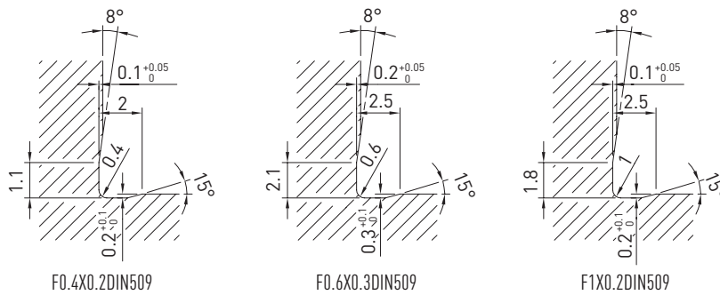
Fig. 3.8 Recommended recess dimensioning of "R" Fig. 3.7 according to DIN 509
