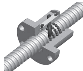
Fig. 3.9 External recirculation type nut
