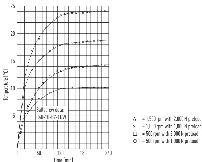
Fig. 3.28 Relationship between operating speed, preload and temperature increase
