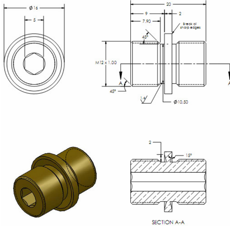
Nipple ZEM M 12 x 1 reference 292403
