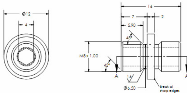
Nipple ZEM M 8 x 1 reference 292401
