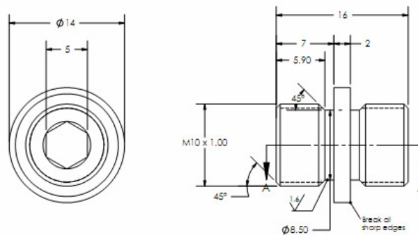
Nipple ZEM M 10 x 1 reference 292402
