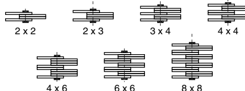
Plate Lacing
